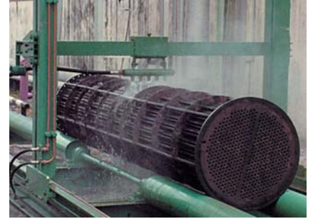
External cleaning of a heat exchanger with the Pipemaster
