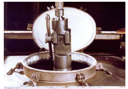
Vessel cleaning with a tank cleaning unit deployed by a customised device
